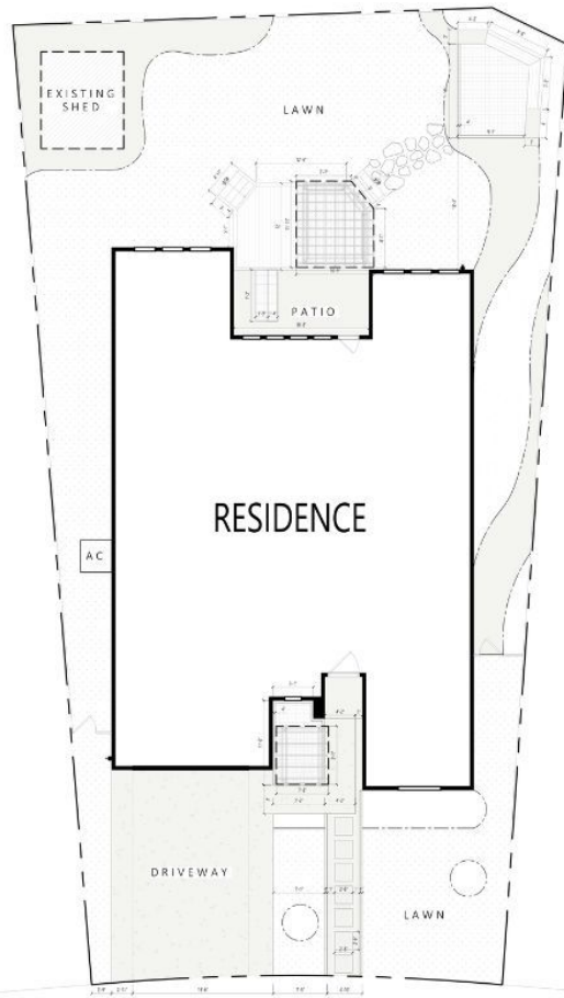
A HARDSCAPE MATERIALS PLAN LS-03 SCALE 1/8"=1'
